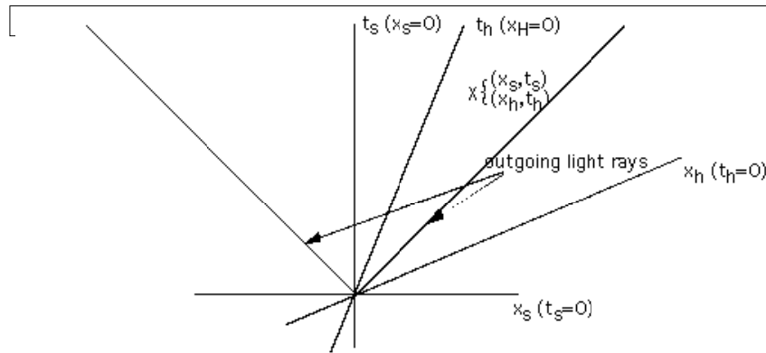
Figure 10.6: Construction of coordinate axis for a relatively moving observer: Harry and Sally have a relative velocity, v , with Harry moving to increasing x to Sally. They both agree to label the event of their coincidence as (0, 0) . His time axis, his x_h = 0 line, is a straight line through the origin with slope \frac{1}{v} and his x axis, his t_h = 0 line, also passes through the origin but has slope \frac{v}{c^2} .
